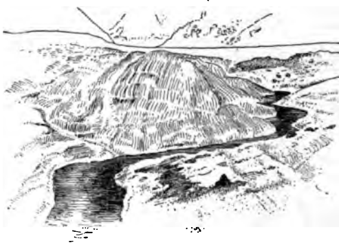
FIG. 427. — Superglacial stream upon the Great Aletsch glacier.
